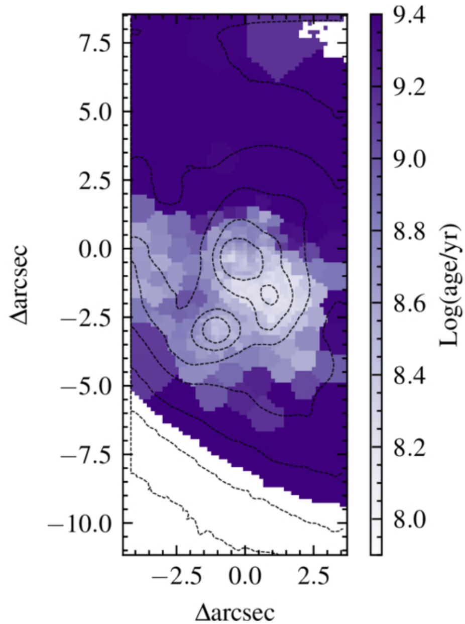
Figure 5. from Yuanze Ding et al 2026 Astrophys. J. 1002 doi:10.3847/1538-4357/ae5643 https://dx.doi.org/10.3847/1538-4357/ae5643 © 2026. The Author(s). Published by the American Astronomical Society.
