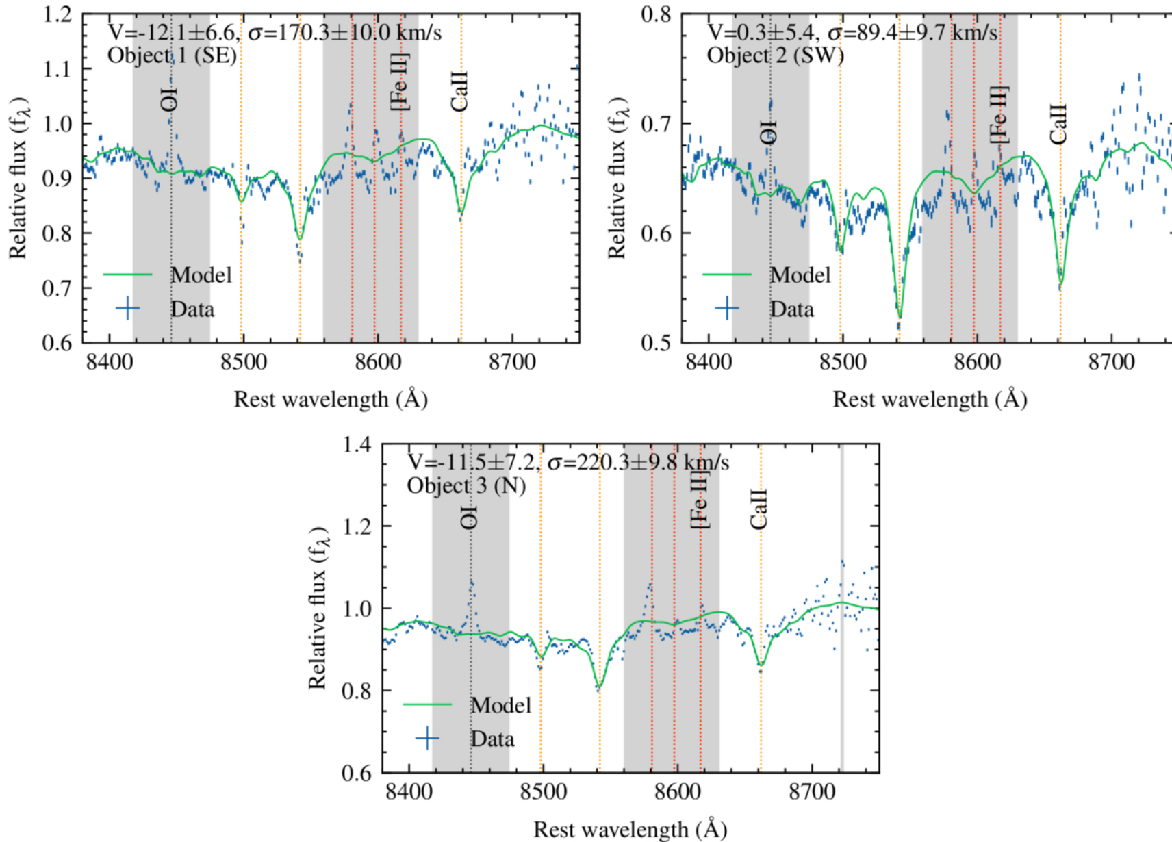
Figure 4. from Yuanze Ding et al 2026 Astrophys. J. 1002 doi:10.3847/1538-4357/ae5643 https://dx.doi.org/10.3847/1538-4357/ae5643 © 2026. The Author(s). Published by the American Astronomical Society.
