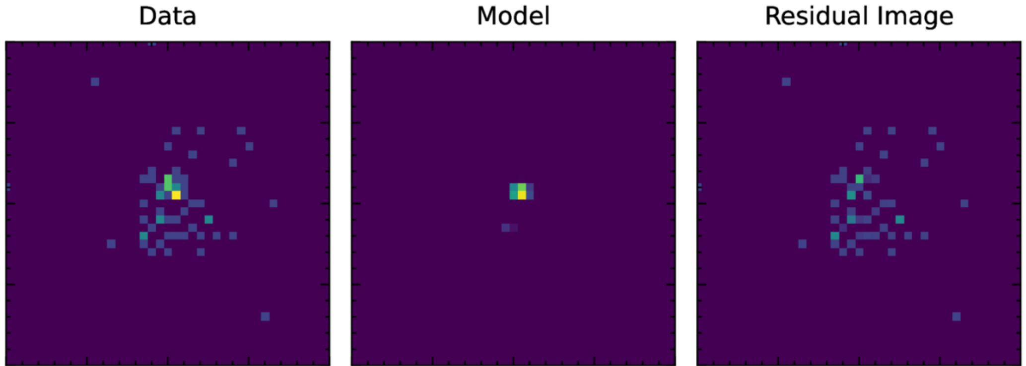
Figure 3. from Yuanze Ding et al 2026 Astrophys. J. 1002 doi:10.3847/1538-4357/ae5643 https://dx.doi.org/10.3847/1538-4357/ae5643 © 2026. The Author(s). Published by the American Astronomical Society.
