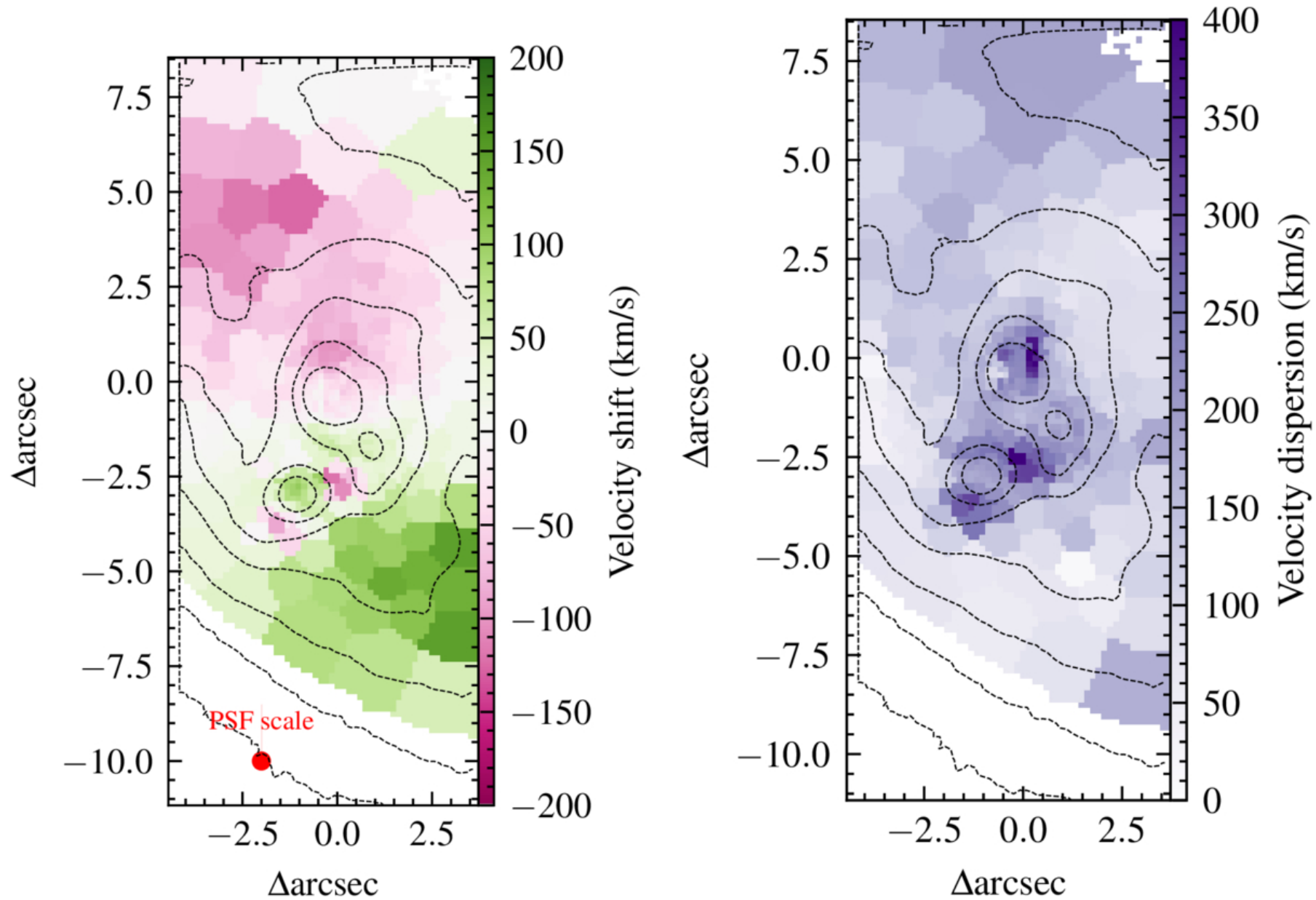
Figure A1. from Yuanze Ding et al 2026 Astrophys. J. 1002 doi:10.3847/1538-4357/ae5643 https://dx.doi.org/10.3847/1538-4357/ae5643 © 2026. The Author(s). Published by the American Astronomical Society.
