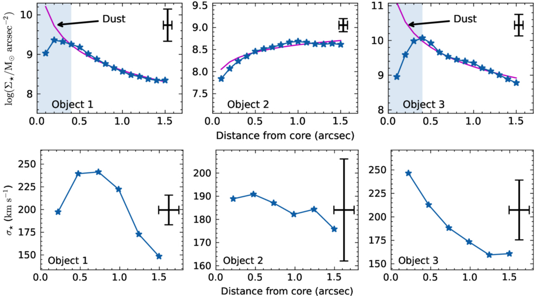
Figure 15. from Yuanze Ding et al 2026 Astrophys. J. 1002 doi:10.3847/1538-4357/ae5643 https://dx.doi.org/10.3847/1538-4357/ae5643 © 2026. The Author(s). Published by the American Astronomical Society.
