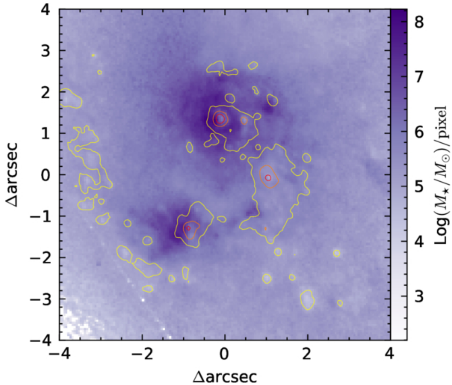
Figure 14. from Yuanze Ding et al 2026 Astrophys. J. 1002 doi:10.3847/1538-4357/ae5643 https://dx.doi.org/10.3847/1538-4357/ae5643 © 2026. The Author(s). Published by the American Astronomical Society.
