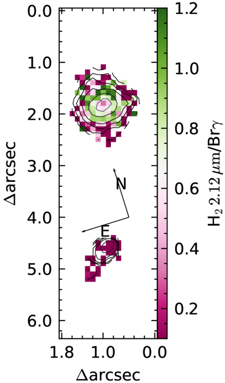
Figure 11. from Yuanze Ding et al 2026 Astrophys. J. 1002 doi:10.3847/1538-4357/ae5643 https://dx.doi.org/10.3847/1538-4357/ae5643 © 2026. The Author(s). Published by the American Astronomical Society.
