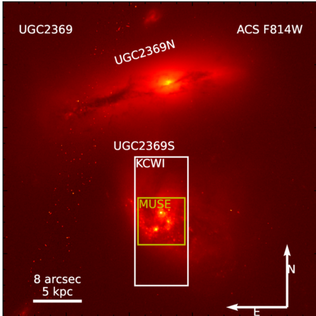
Figure 1. from Yuanze Ding et al 2026 Astrophys. J. 1002 doi:10.3847/1538-4357/ae5643 https://dx.doi.org/10.3847/1538-4357/ae5643 © 2026. The Author(s). Published by the American Astronomical Society.
