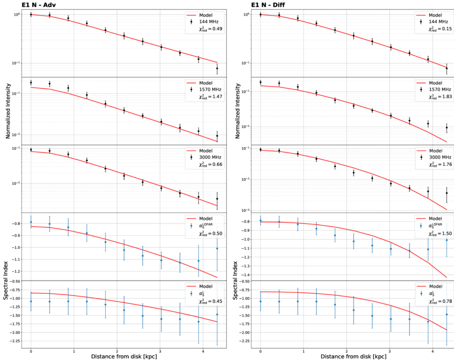
Figure 8. from Jianghui Xu et al 2026 Astrophys. J. 1001 doi:10.3847/1538-4357/ae5636 https://dx.doi.org/10.3847/1538-4357/ae5636 © 2026. The Author(s). Published by the American Astronomical Society.
