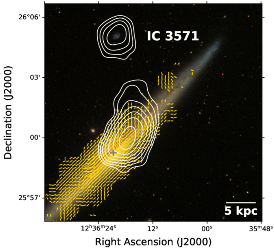
Figure 10. from Jianghui Xu et al 2026 Astrophys. J. 1001 doi:10.3847/1538-4357/ae5636 https://dx.doi.org/10.3847/1538-4357/ae5636 © 2026. The Author(s). Published by the American Astronomical Society.
