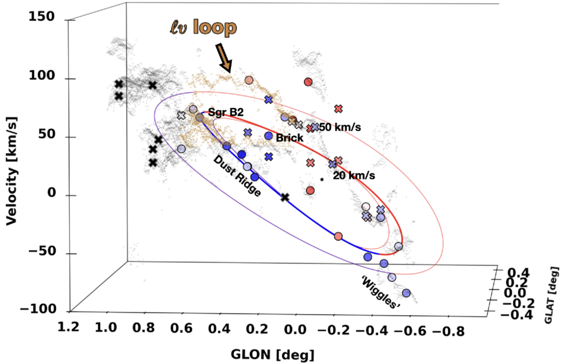
Figure 8. from Dani R. Lipman et al 2026 Astrophys. J. 1002 doi:10.3847/1538-4357/ae561f https://dx.doi.org/10.3847/1538-4357/ae561f © 2026. The Author(s). Published by the American Astronomical Society.
