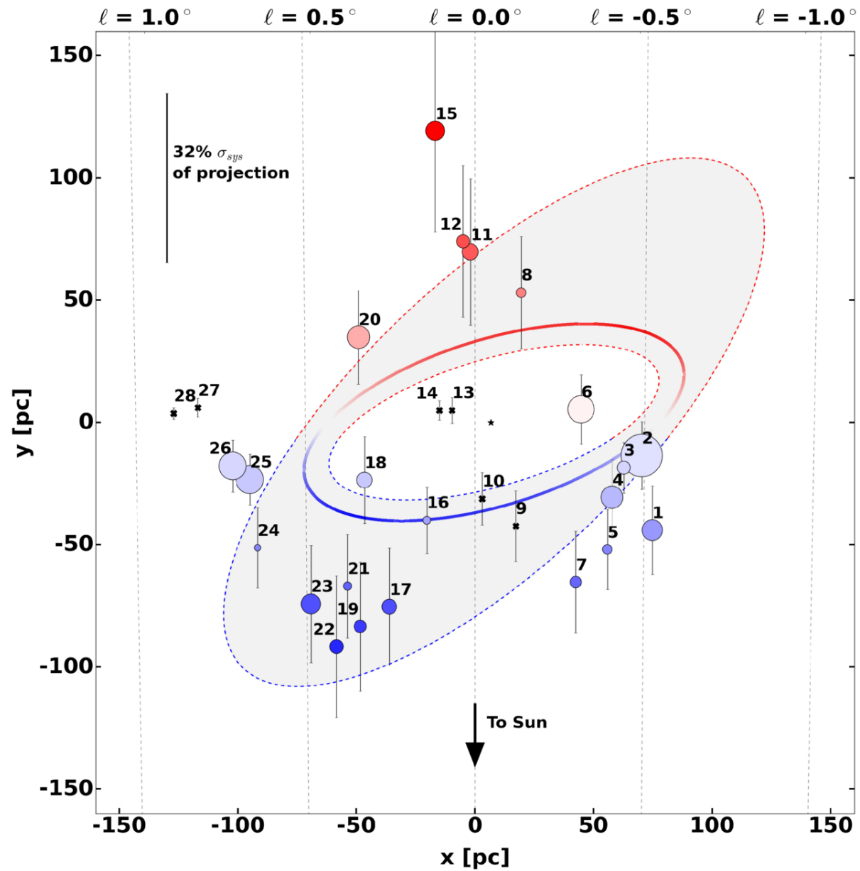
Figure 6. from Dani R. Lipman et al 2026 Astrophys. J. 1002 doi:10.3847/1538-4357/ae561f https://dx.doi.org/10.3847/1538-4357/ae561f © 2026. The Author(s). Published by the American Astronomical Society.
