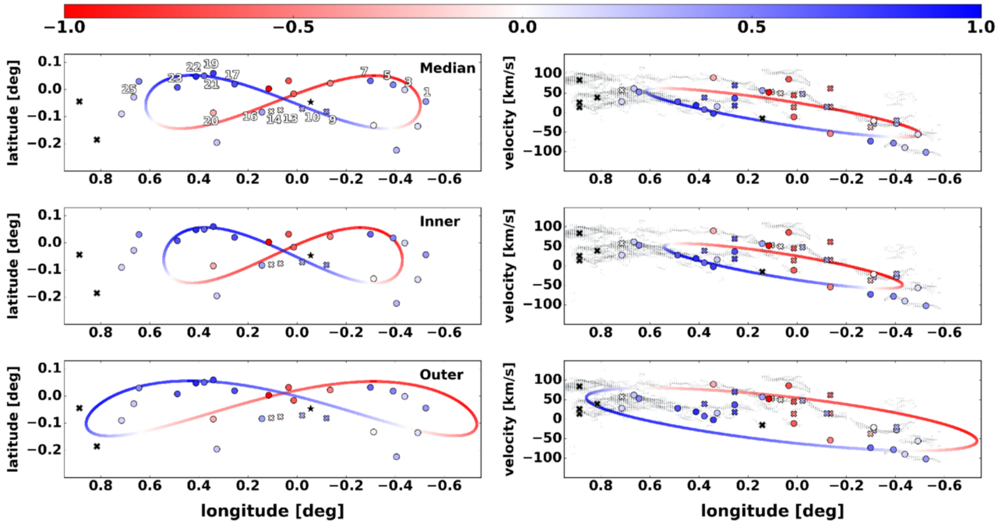
Figure 5. from Dani R. Lipman et al 2026 Astrophys. J. 1002 doi:10.3847/1538-4357/ae561f https://dx.doi.org/10.3847/1538-4357/ae561f © 2026. The Author(s). Published by the American Astronomical Society.
