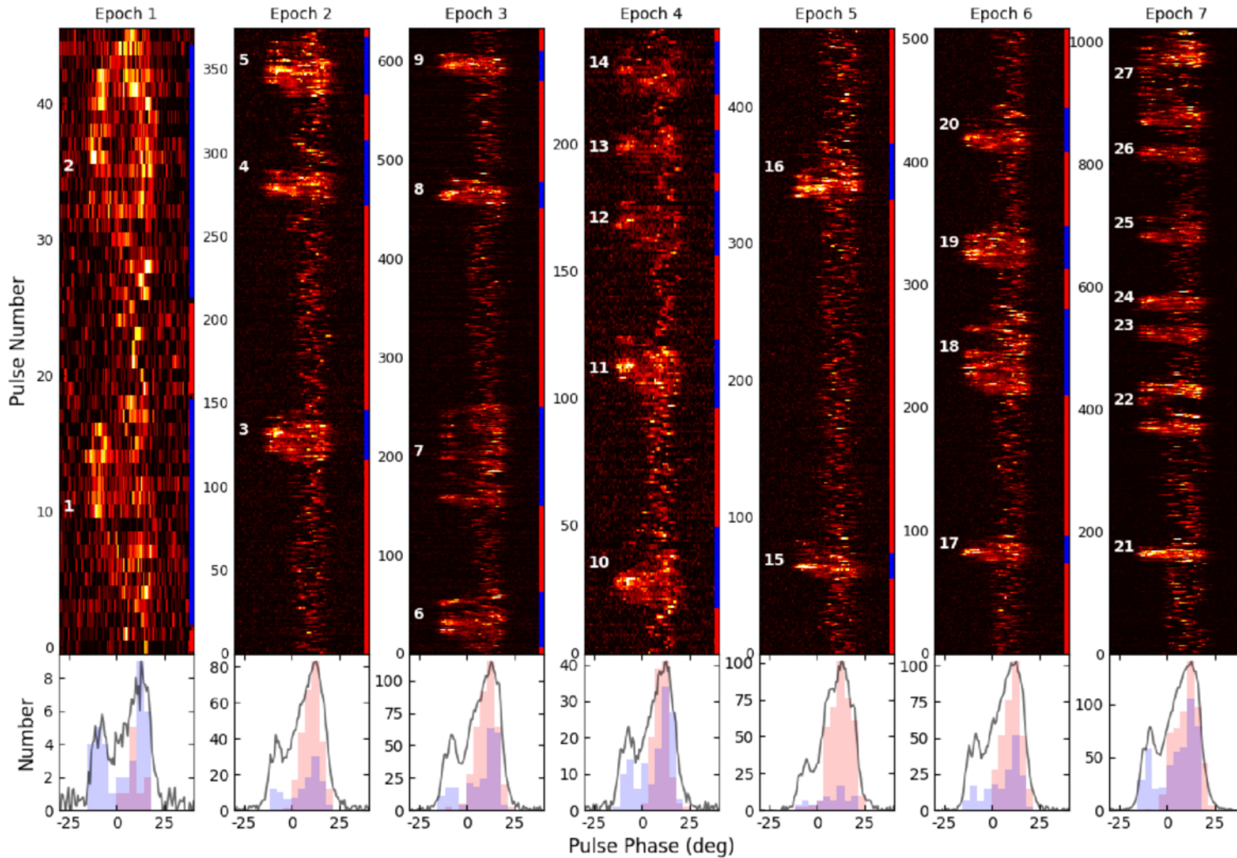
Figure 6. from Xin Xu et al 2026 Astrophys. J. 1002 doi:10.3847/1538-4357/ae5532 https://dx.doi.org/10.3847/1538-4357/ae5532 © 2026. The Author(s). Published by the American Astronomical Society.
