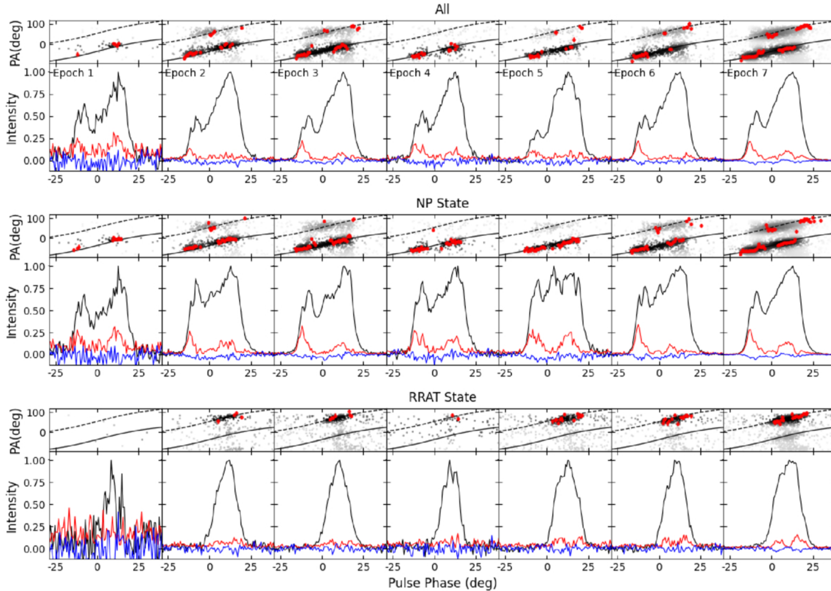
Figure 2. from Xin Xu et al 2026 Astrophys. J. 1002 doi:10.3847/1538-4357/ae5532 https://dx.doi.org/10.3847/1538-4357/ae5532 © 2026. The Author(s). Published by the American Astronomical Society.
