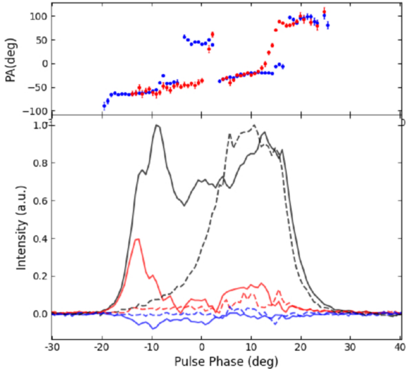
Figure 11. from Xin Xu et al 2026 Astrophys. J. 1002 doi:10.3847/1538-4357/ae5532 https://dx.doi.org/10.3847/1538-4357/ae5532 © 2026. The Author(s). Published by the American Astronomical Society.
