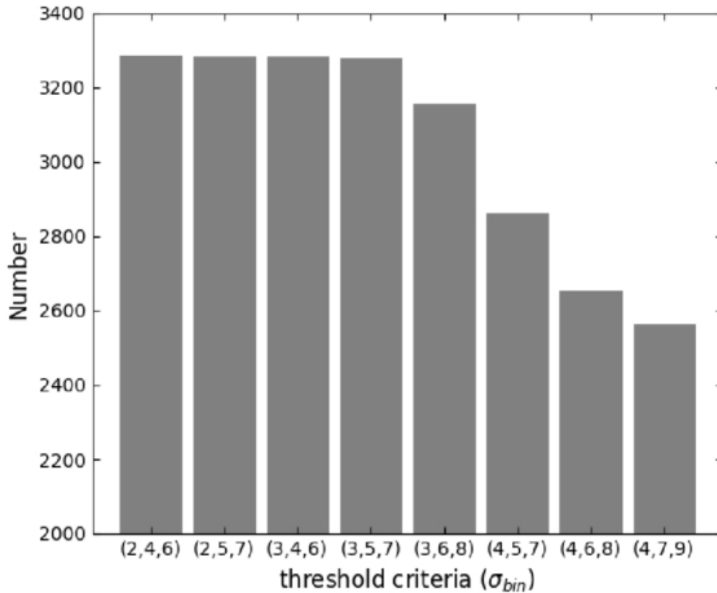
Figure 1. from Xin Xu et al 2026 Astrophys. J. 1002 doi:10.3847/1538-4357/ae5532 https://dx.doi.org/10.3847/1538-4357/ae5532 © 2026. The Author(s). Published by the American Astronomical Society.
