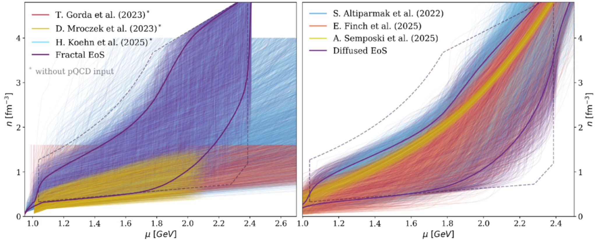
Figure 9. from Tyler Gorda et al 2026 Astrophys. J. 1002 doi:10.3847/1538-4357/ae552a https://dx.doi.org/10.3847/1538-4357/ae552a © 2026. The Author(s). Published by the American Astronomical Society.
