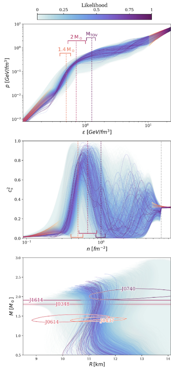
Figure 6. from Tyler Gorda et al 2026 Astrophys. J. 1002 doi:10.3847/1538-4357/ae552a https://dx.doi.org/10.3847/1538-4357/ae552a © 2026. The Author(s). Published by the American Astronomical Society.
