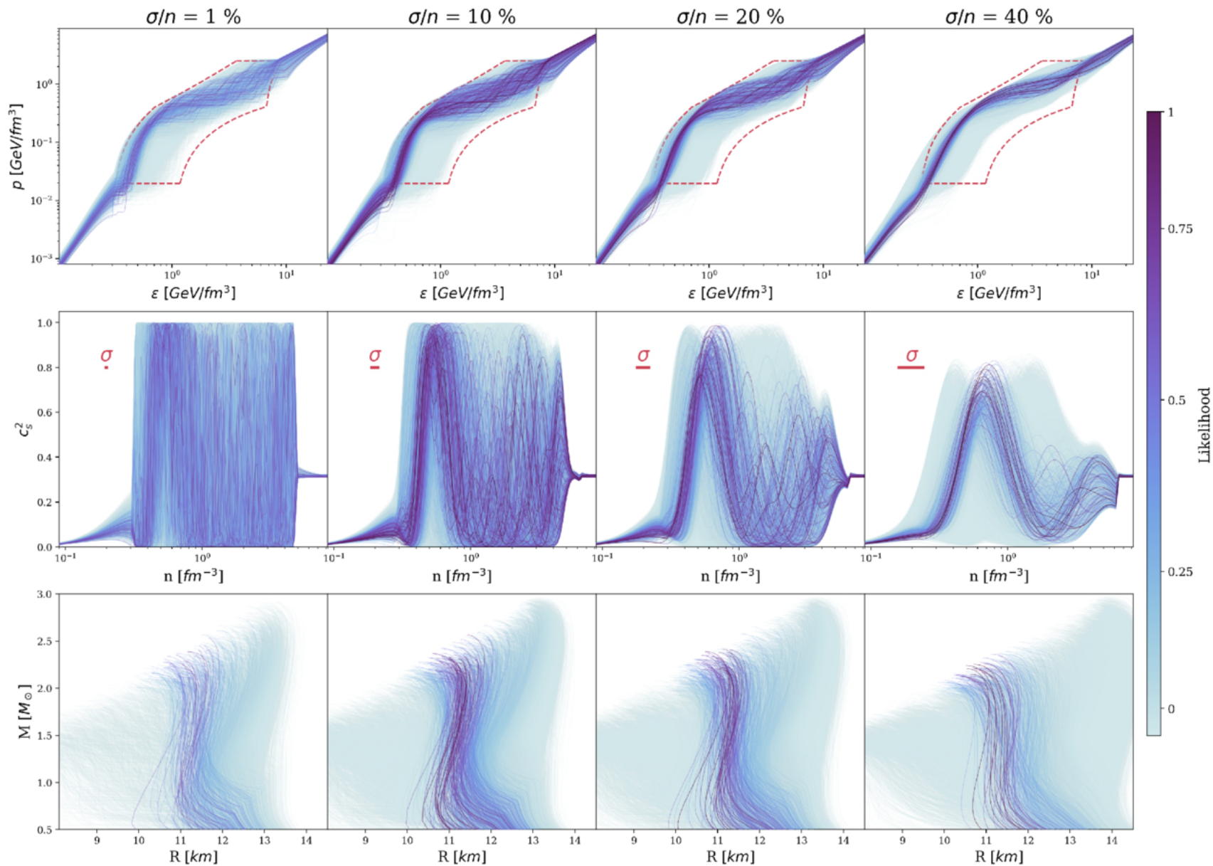
Figure 5. from Tyler Gorda et al 2026 Astrophys. J. 1002 doi:10.3847/1538-4357/ae552a https://dx.doi.org/10.3847/1538-4357/ae552a © 2026. The Author(s). Published by the American Astronomical Society.
