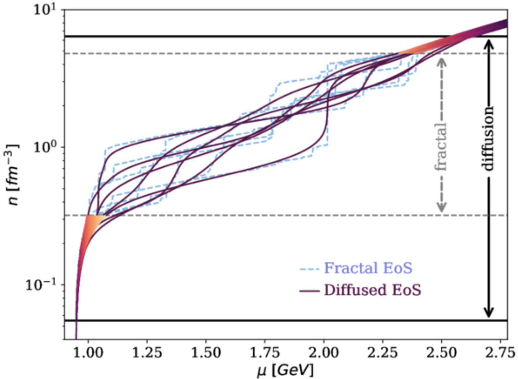
Figure 4. from Tyler Gorda et al 2026 Astrophys. J. 1002 doi:10.3847/1538-4357/ae552a https://dx.doi.org/10.3847/1538-4357/ae552a © 2026. The Author(s). Published by the American Astronomical Society.
