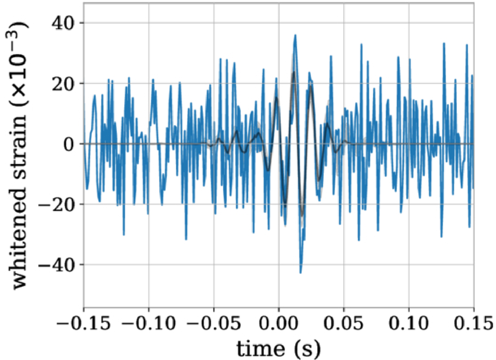
Figure 3. from Shun Yin Cheung et al 2026 Astrophys. J. 1001 doi:10.3847/1538-4357/ae5493 https://dx.doi.org/10.3847/1538-4357/ae5493 © 2026. The Author(s). Published by the American Astronomical Society.
