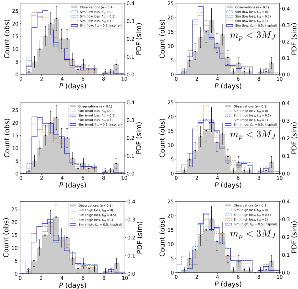
Figure 8. from Grant C. Weldon et al 2026 Astrophys. J. 1001 doi:10.3847/1538-4357/ae548c https://dx.doi.org/10.3847/1538-4357/ae548c © 2026. The Author(s). Published by the American Astronomical Society.
