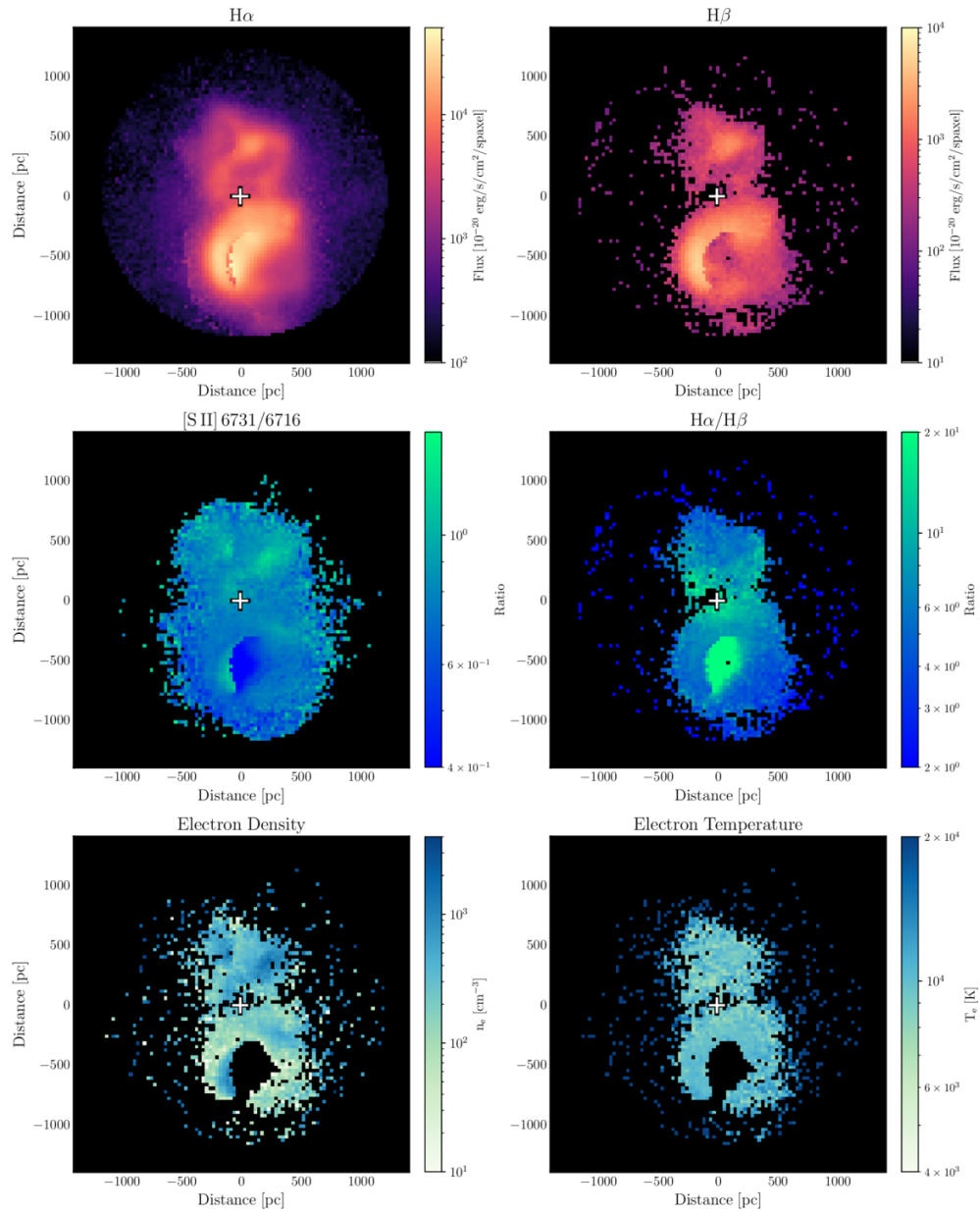
Figure 6. from Sebastian Lopez et al 2026 Astrophys. J. 1001 doi:10.3847/1538-4357/ae5480 https://dx.doi.org/10.3847/1538-4357/ae5480 © 2026. The Author(s). Published by the American Astronomical Society.
