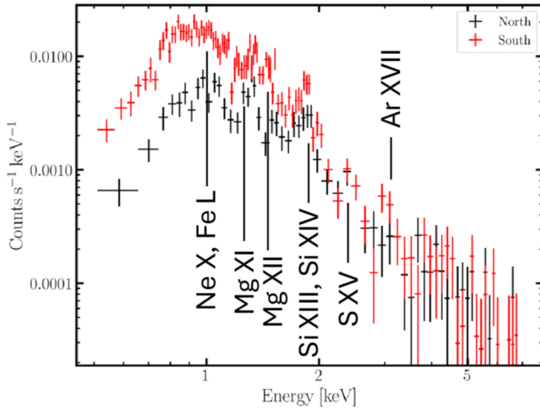
Figure 3. from Sebastian Lopez et al 2026 Astrophys. J. 1001 doi:10.3847/1538-4357/ae5480 https://dx.doi.org/10.3847/1538-4357/ae5480 © 2026. The Author(s). Published by the American Astronomical Society.
