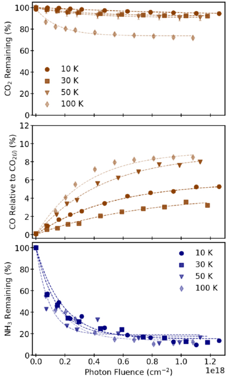
Figure 5. from Alexandra McKinnon et al 2026 Astrophys. J. 1001 doi:10.3847/1538-4357/ae53e1 https://dx.doi.org/10.3847/1538-4357/ae53e1 © 2026. The Author(s). Published by the American Astronomical Society.
