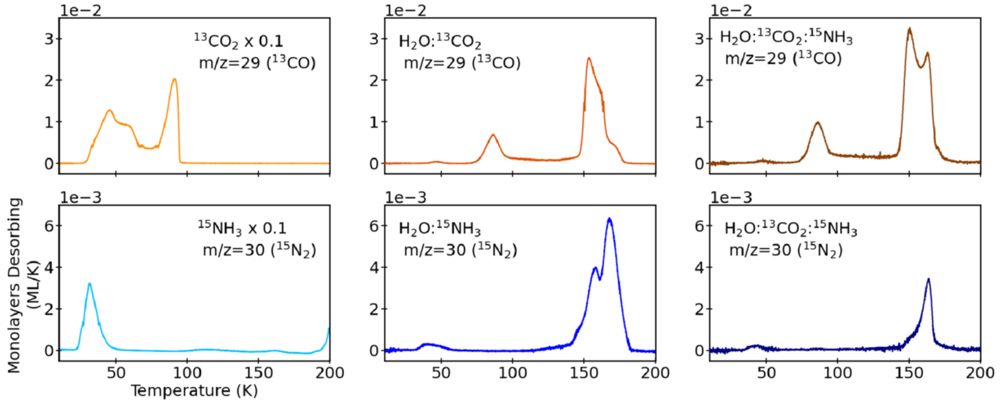
Figure 3. from Alexandra McKinnon et al 2026 Astrophys. J. 1001 doi:10.3847/1538-4357/ae53e1 https://dx.doi.org/10.3847/1538-4357/ae53e1 © 2026. The Author(s). Published by the American Astronomical Society.
