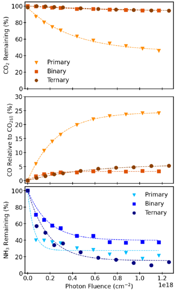
Figure 2. from Alexandra McKinnon et al 2026 Astrophys. J. 1001 doi:10.3847/1538-4357/ae53e1 https://dx.doi.org/10.3847/1538-4357/ae53e1 © 2026. The Author(s). Published by the American Astronomical Society.
