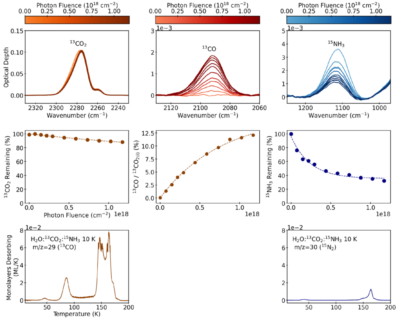
Figure 15. from Alexandra McKinnon et al 2026 Astrophys. J. 1001 doi:10.3847/1538-4357/ae53e1 https://dx.doi.org/10.3847/1538-4357/ae53e1 © 2026. The Author(s). Published by the American Astronomical Society.
