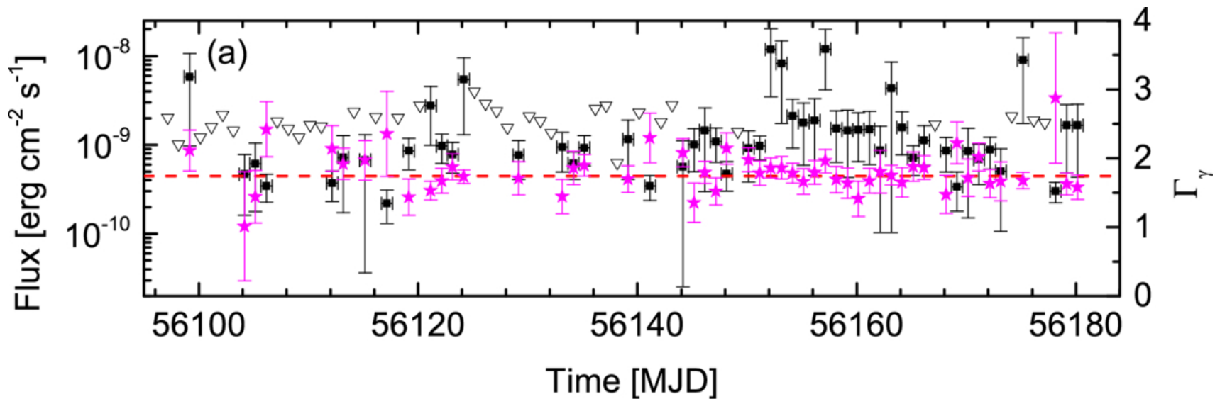
Figure 3. from Rui-Qi Huang et al 2026 Astrophys. J. 1001 doi:10.3847/1538-4357/ae53de https://dx.doi.org/10.3847/1538-4357/ae53de © 2026. The Author(s). Published by the American Astronomical Society.
