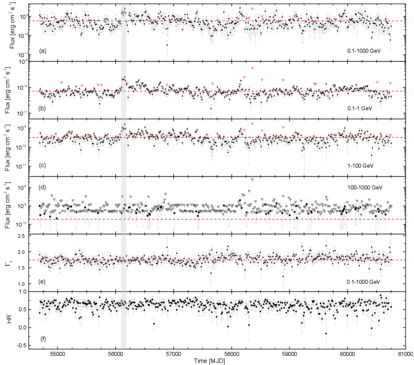
Figure 2. from Rui-Qi Huang et al 2026 Astrophys. J. 1001 doi:10.3847/1538-4357/ae53de https://dx.doi.org/10.3847/1538-4357/ae53de © 2026. The Author(s). Published by the American Astronomical Society.
