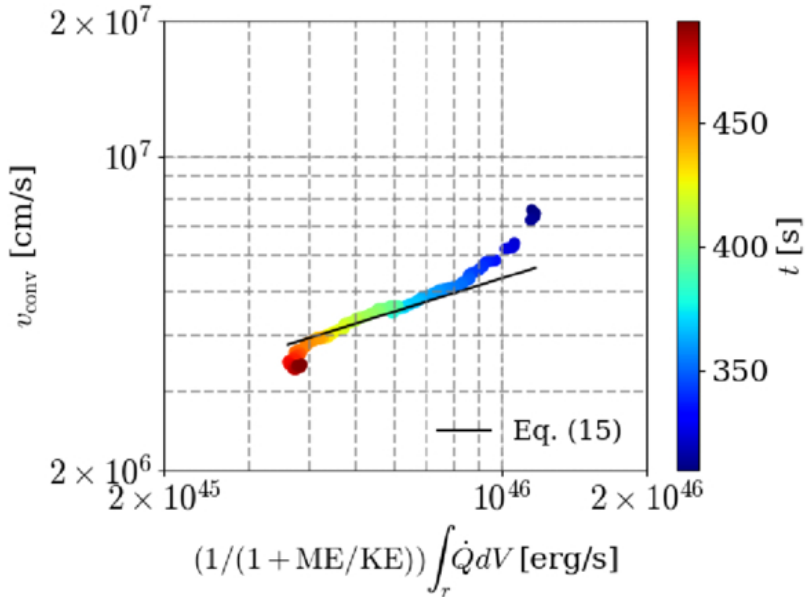
Figure 4. from Ryota Shimada et al 2026 Astrophys. J. 1002 doi:10.3847/1538-4357/ae53da https://dx.doi.org/10.3847/1538-4357/ae53da © 2026. The Author(s). Published by the American Astronomical Society.
