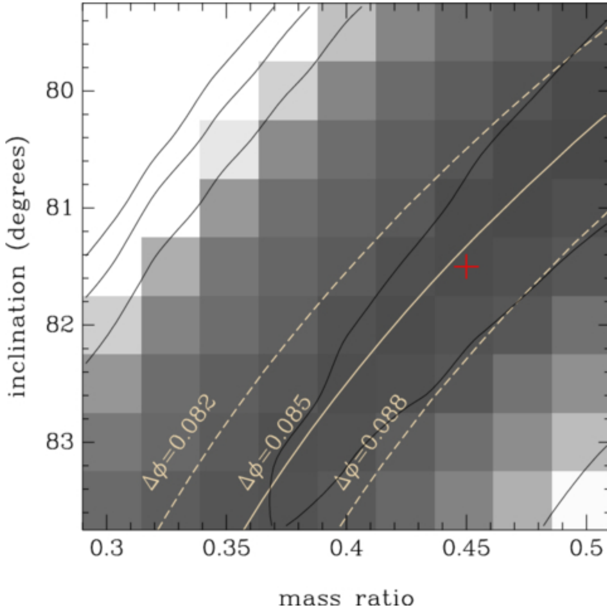
Figure 2. from Raymundo Baptista et al 2026 Astrophys. J. 1001 doi:10.3847/1538-4357/ae5232 https://dx.doi.org/10.3847/1538-4357/ae5232 © 2026. The Author(s). Published by the American Astronomical Society.
