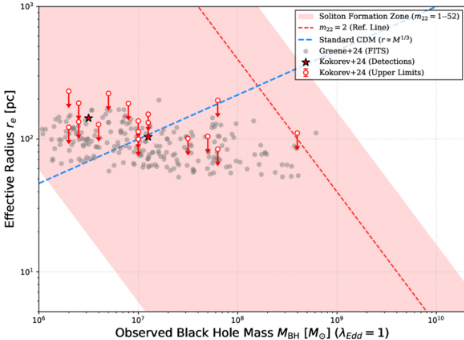
Figure 4: Formation Boundary ( m_{22}=1-52 )
