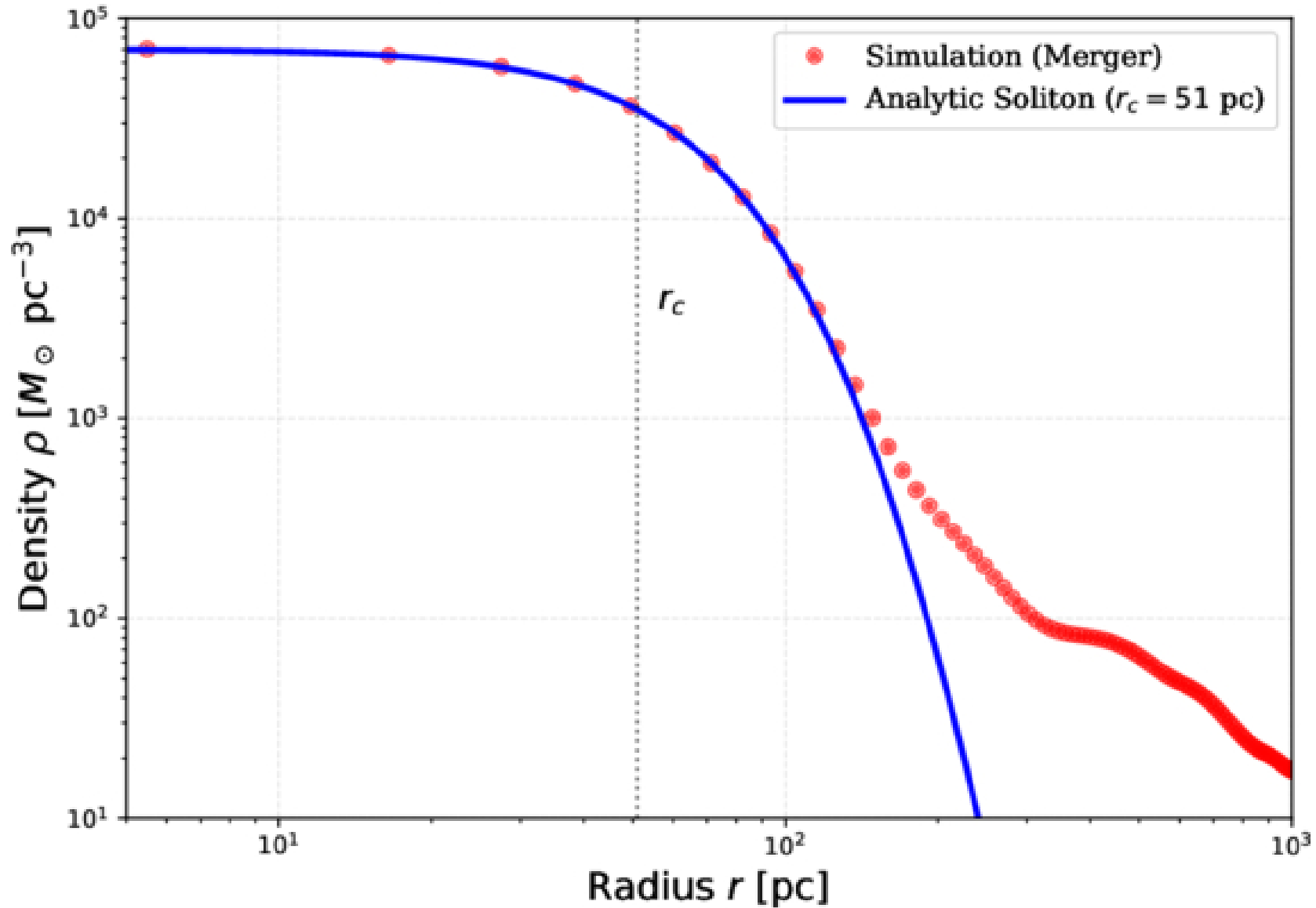
Figure 3: Soliton Profile Validation
