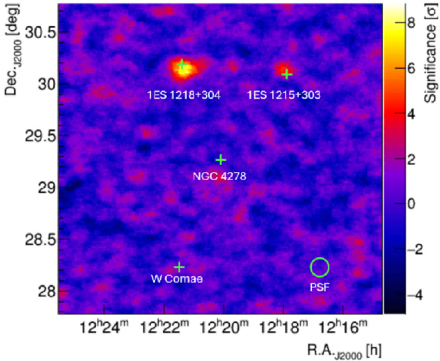
Figure 1. from A. Archer et al 2026 Astrophys. J. 1001 doi:10.3847/1538-4357/ae5226 https://dx.doi.org/10.3847/1538-4357/ae5226 © 2026. The Author(s). Published by the American Astronomical Society.
