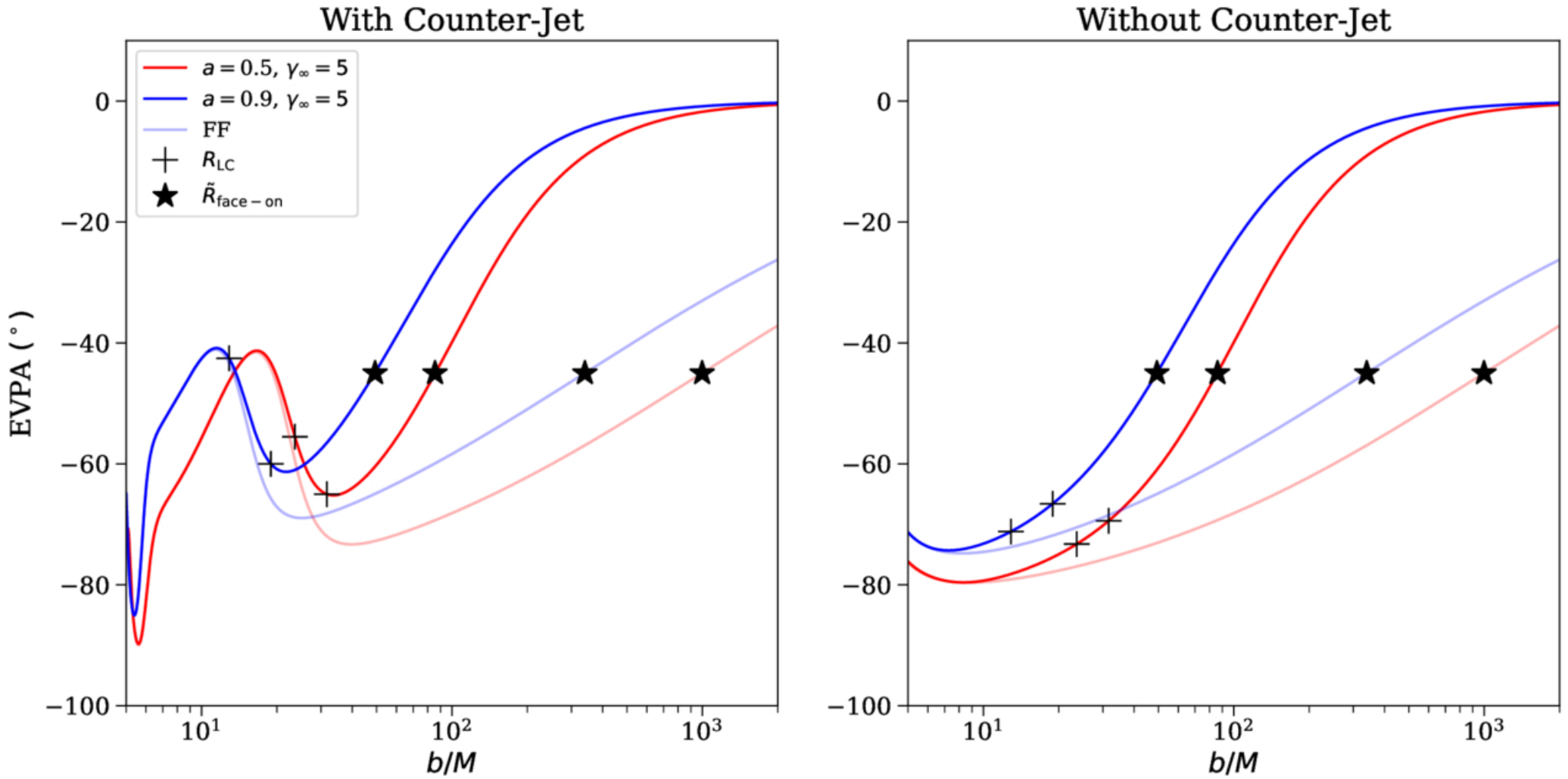
Figure 3. from Z. Gelles et al 2026 Astrophys. J. 1001 doi:10.3847/1538-4357/ae5223 https://dx.doi.org/10.3847/1538-4357/ae5223 © 2026. The Author(s). Published by the American Astronomical Society.
