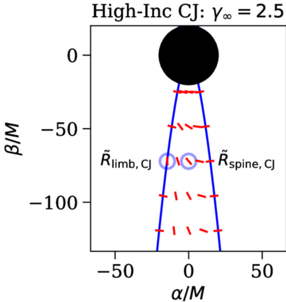
Figure 18. from Z. Gelles et al 2026 Astrophys. J. 1001 doi:10.3847/1538-4357/ae5223 https://dx.doi.org/10.3847/1538-4357/ae5223 © 2026. The Author(s). Published by the American Astronomical Society.
