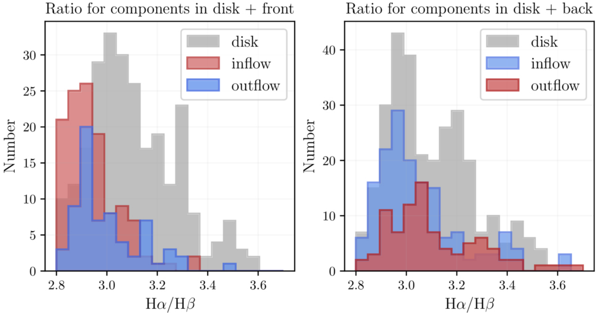
Figure 6. from Meghna Sitaram et al 2026 Astrophys. J. 1001 doi:10.3847/1538-4357/ae5222 https://dx.doi.org/10.3847/1538-4357/ae5222 © 2026. The Author(s). Published by the American Astronomical Society.
