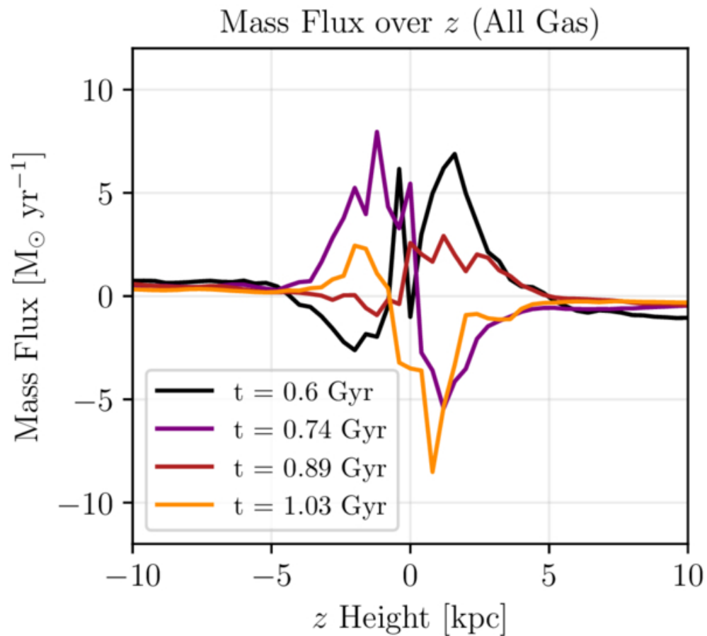
Figure 3. from Meghna Sitaram et al 2026 Astrophys. J. 1001 doi:10.3847/1538-4357/ae5222 https://dx.doi.org/10.3847/1538-4357/ae5222 © 2026. The Author(s). Published by the American Astronomical Society.
