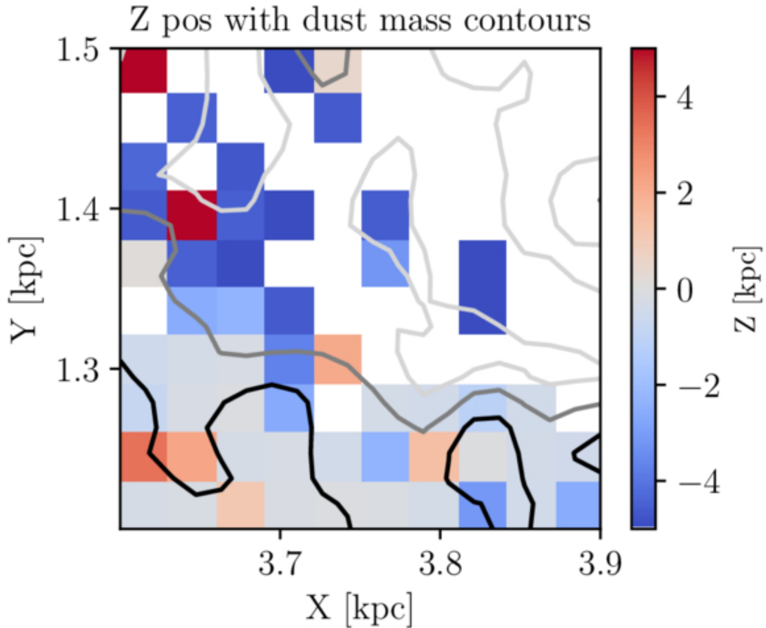
Figure 10. from Meghna Sitaram et al 2026 Astrophys. J. 1001 doi:10.3847/1538-4357/ae5222 https://dx.doi.org/10.3847/1538-4357/ae5222 © 2026. The Author(s). Published by the American Astronomical Society.
