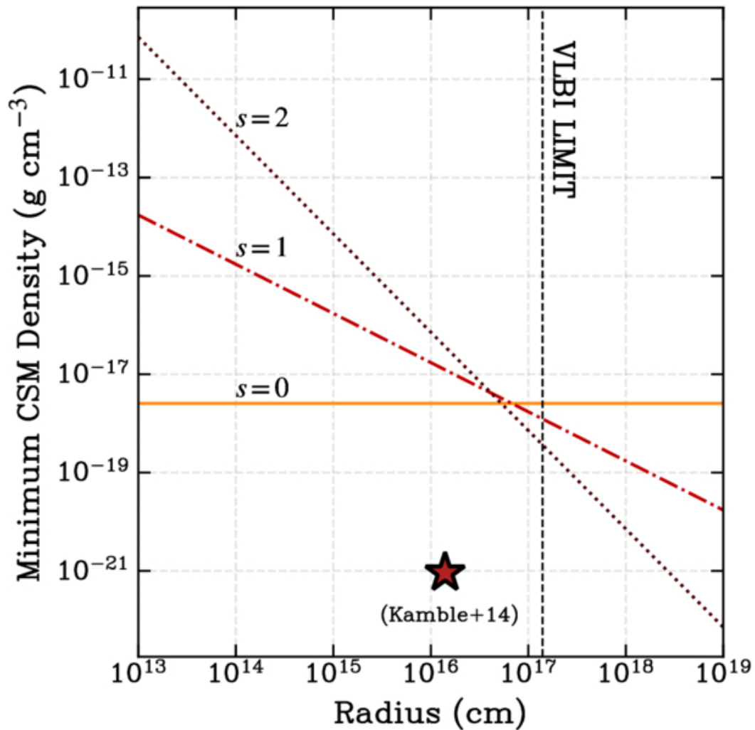
Figure 6. from Mattias Lazda et al 2026 Astrophys. J. 1001 doi:10.3847/1538-4357/ae517f https://dx.doi.org/10.3847/1538-4357/ae517f © 2026. The Author(s). Published by the American Astronomical Society.
