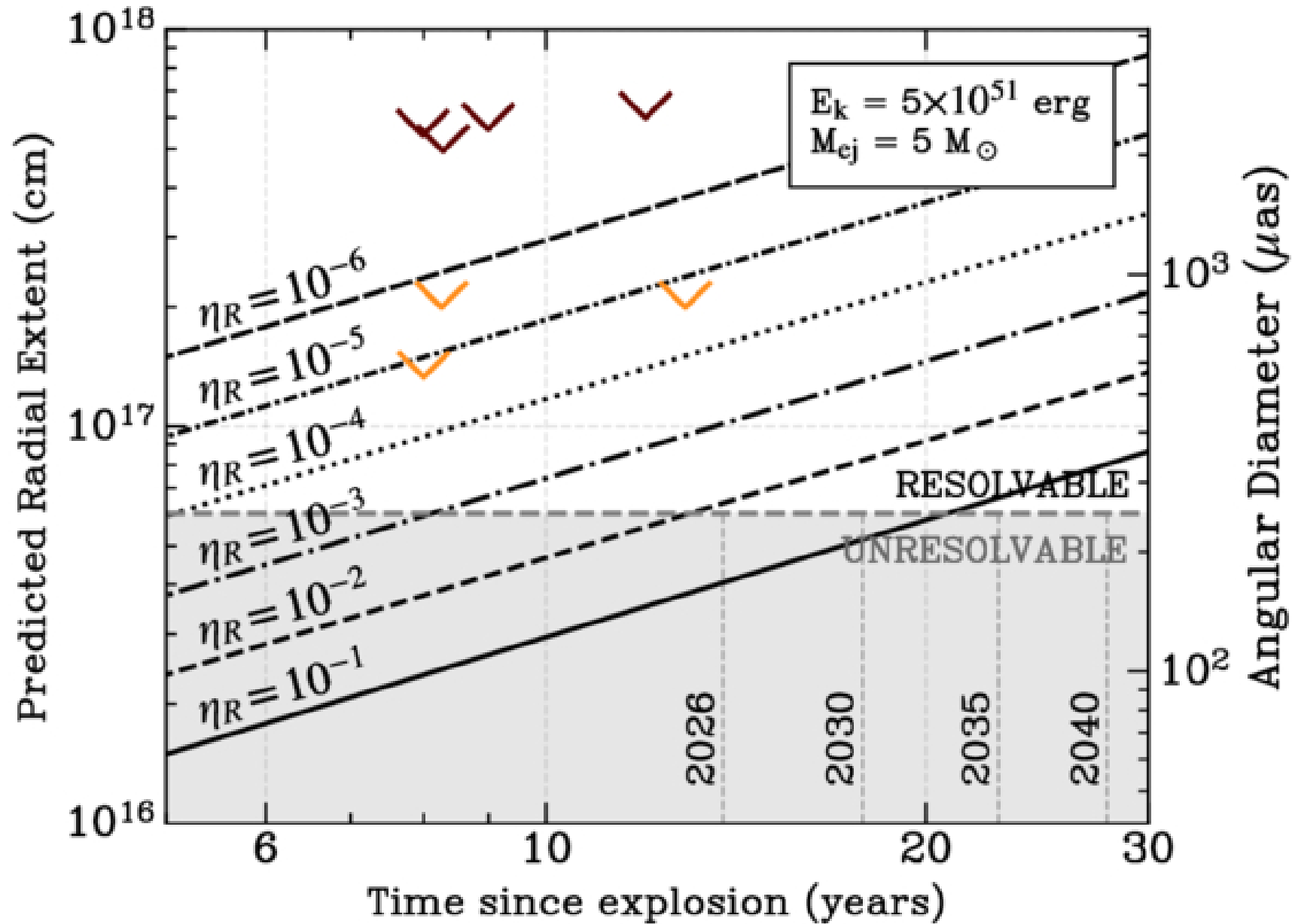
Figure 5. from Mattias Lazda et al 2026 Astrophys. J. 1001 doi:10.3847/1538-4357/ae517f https://dx.doi.org/10.3847/1538-4357/ae517f © 2026. The Author(s). Published by the American Astronomical Society.
