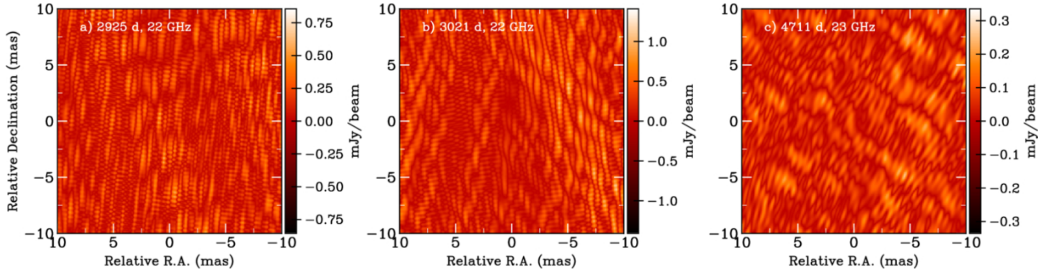
Figure 10. from Mattias Lazda et al 2026 Astrophys. J. 1001 doi:10.3847/1538-4357/ae517f https://dx.doi.org/10.3847/1538-4357/ae517f © 2026. The Author(s). Published by the American Astronomical Society.
