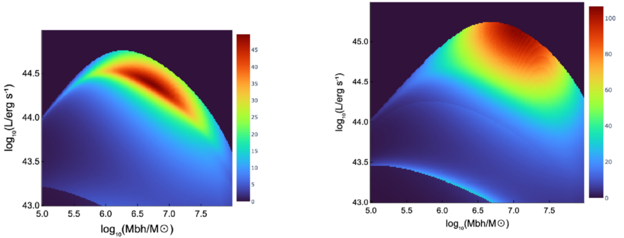
Figure 6. from Tsvi Piran et al 2026 Astrophys. J. 1001 doi:10.3847/1538-4357/ae50ff https://dx.doi.org/10.3847/1538-4357/ae50ff © 2026. The Author(s). Published by the American Astronomical Society.
