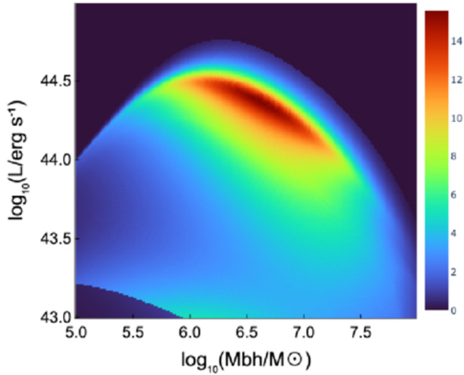
Figure 5. from Tsvi Piran et al 2026 Astrophys. J. 1001 doi:10.3847/1538-4357/ae50ff https://dx.doi.org/10.3847/1538-4357/ae50ff © 2026. The Author(s). Published by the American Astronomical Society.
