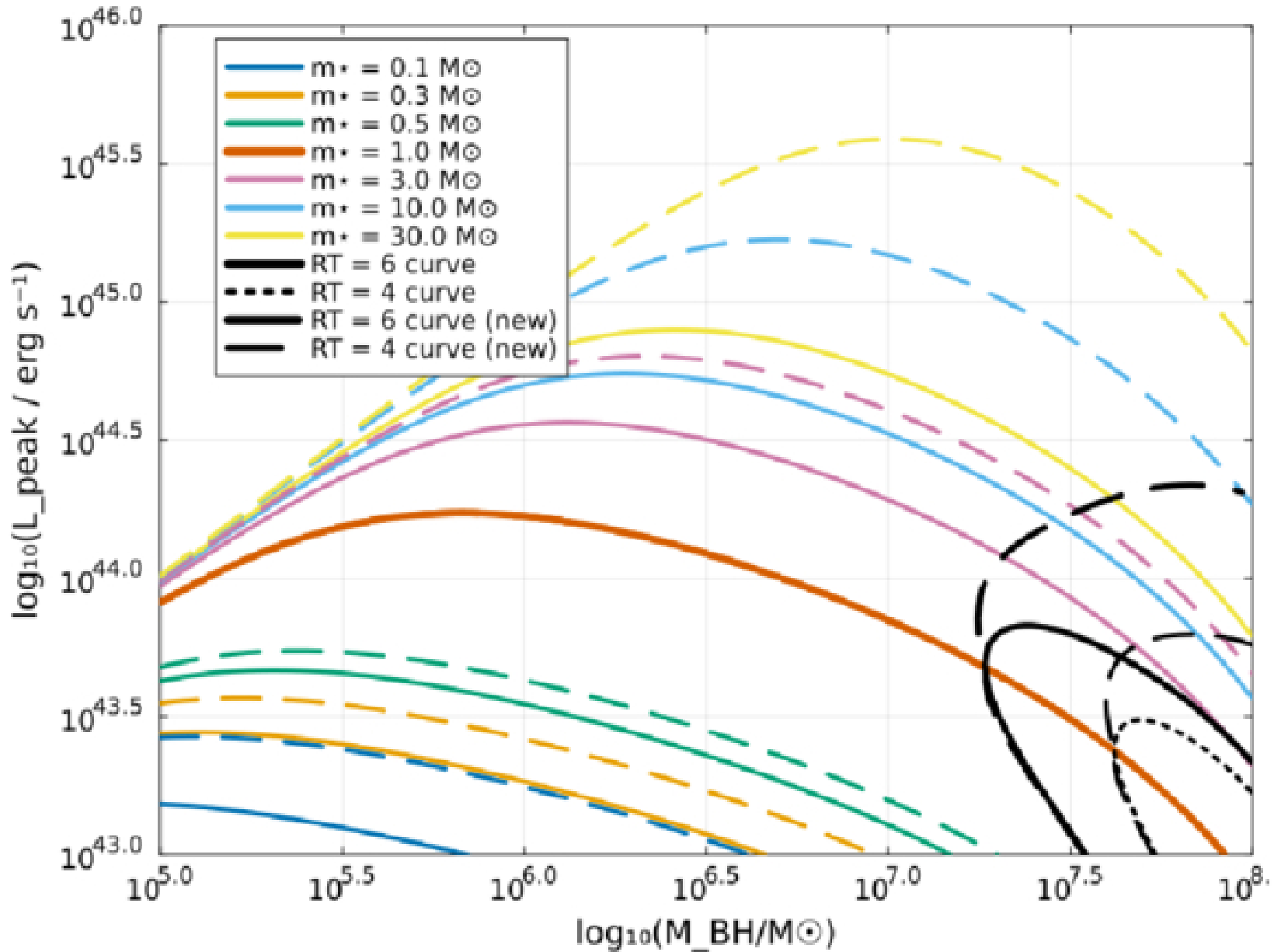
Figure 2. from Tsvi Piran et al 2026 Astrophys. J. 1001 doi:10.3847/1538-4357/ae50ff https://dx.doi.org/10.3847/1538-4357/ae50ff © 2026. The Author(s). Published by the American Astronomical Society.
