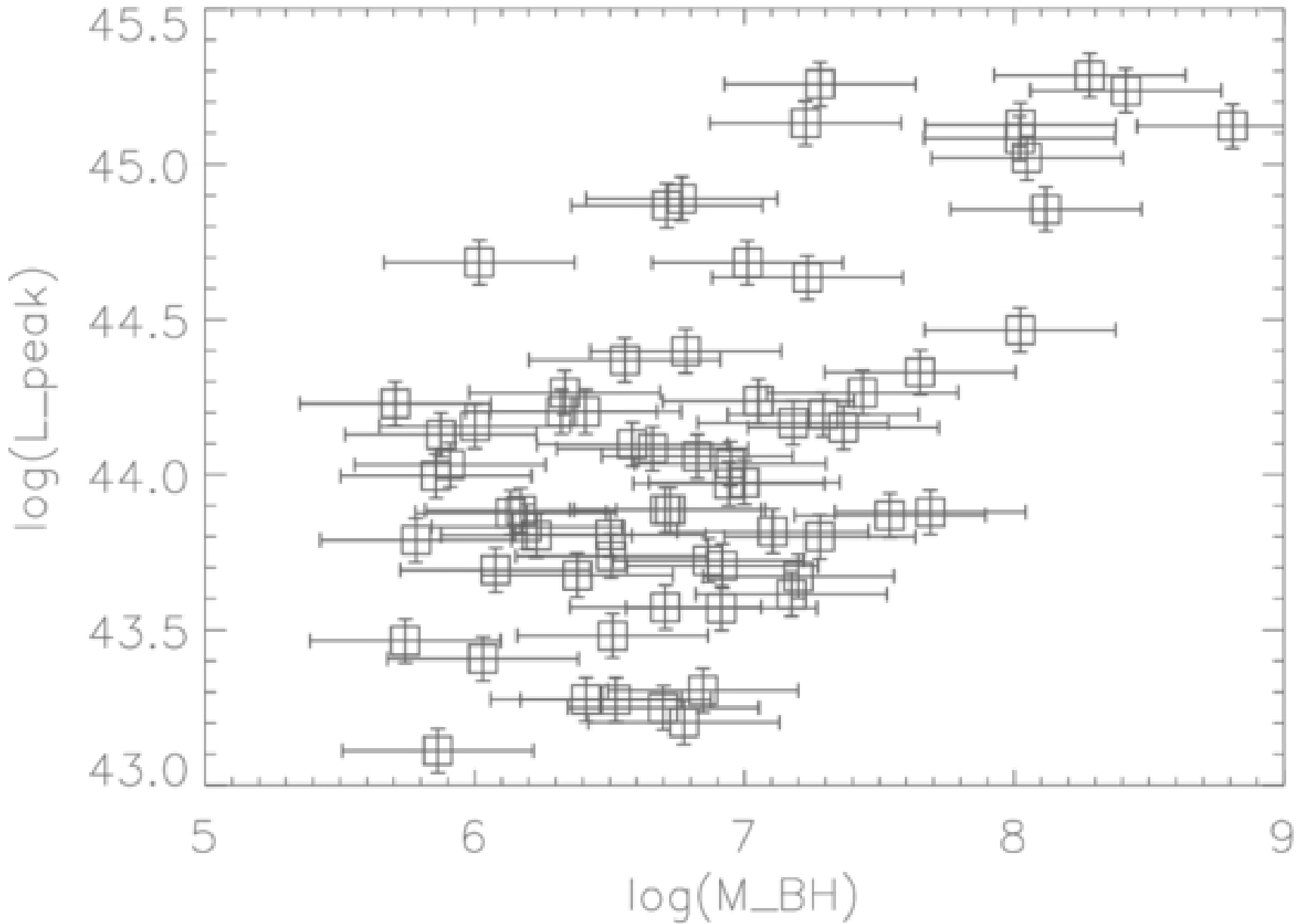
Figure 1. from Tsvi Piran et al 2026 Astrophys. J. 1001 doi:10.3847/1538-4357/ae50ff https://dx.doi.org/10.3847/1538-4357/ae50ff © 2026. The Author(s). Published by the American Astronomical Society.
