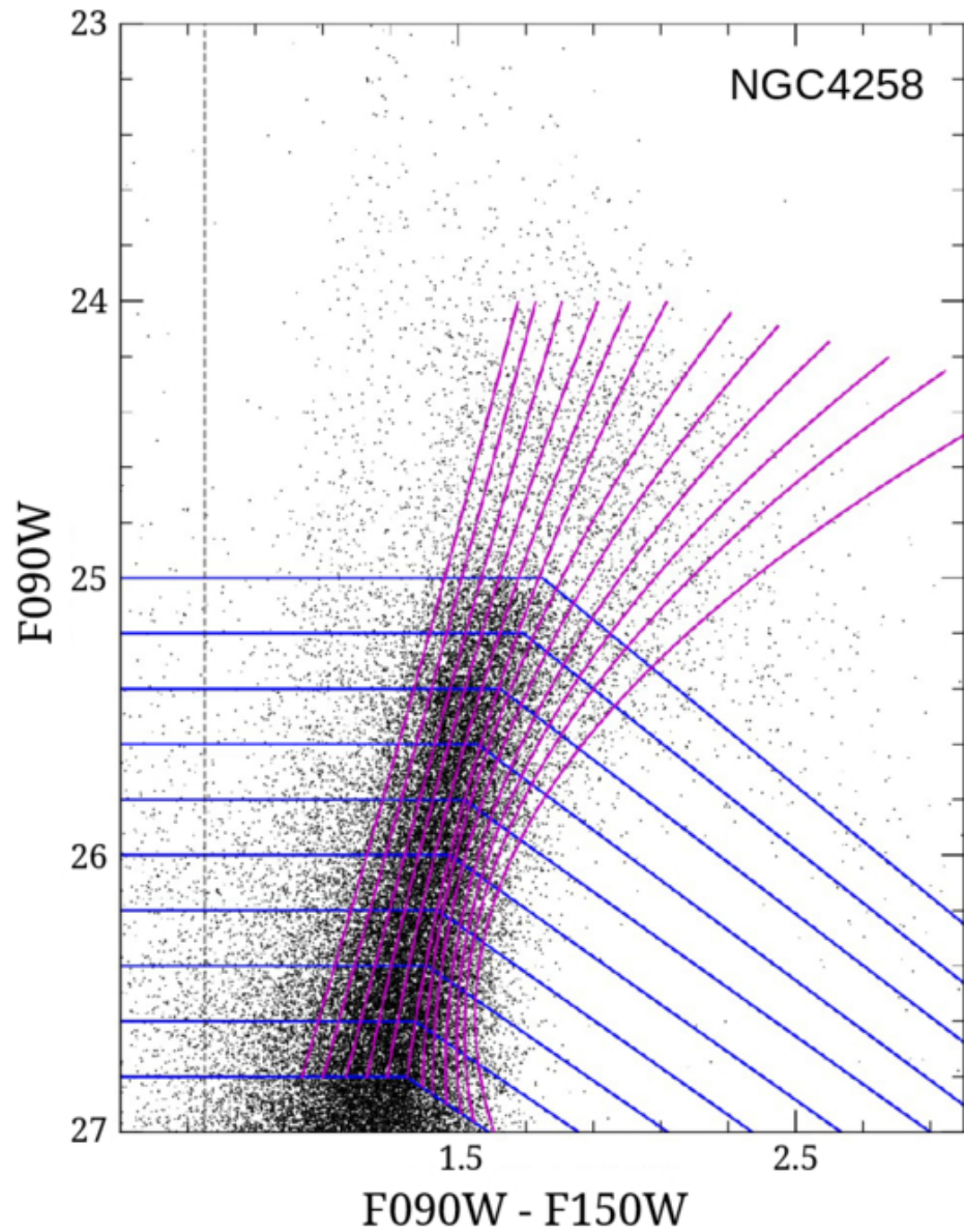
Figure 5. from Maksim I. Chazov et al 2026 Astrophys. J. 1001 doi:10.3847/1538-4357/ae50ed https://dx.doi.org/10.3847/1538-4357/ae50ed © 2026. The Author(s). Published by the American Astronomical Society.
