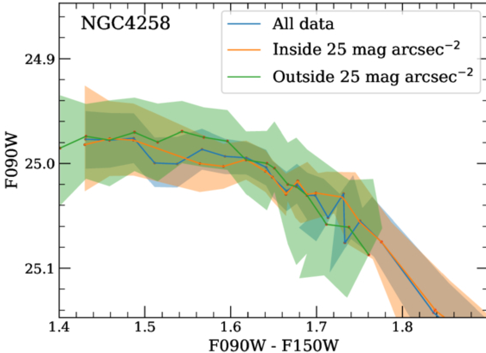
Figure 4. from Maksim I. Chazov et al 2026 Astrophys. J. 1001 doi:10.3847/1538-4357/ae50ed https://dx.doi.org/10.3847/1538-4357/ae50ed © 2026. The Author(s). Published by the American Astronomical Society.
